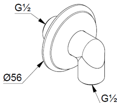
Dimensional drawing
