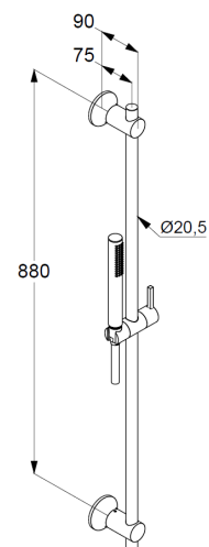
Dimensional drawing
