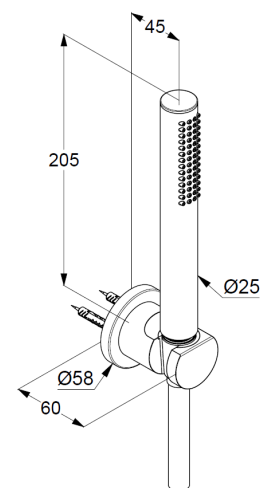
Dimensional drawing
