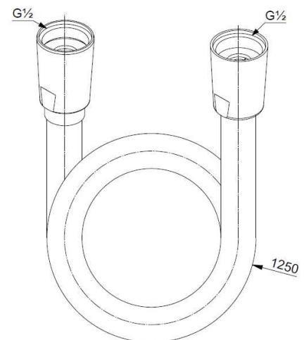
Dimensional drawing
