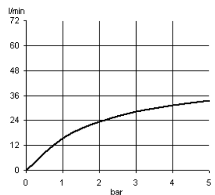
Flow rate diagram
