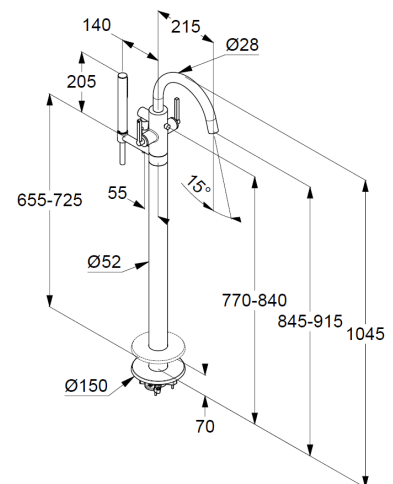
Dimensional drawing
