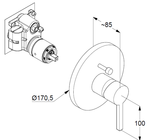
Dimensional drawing
