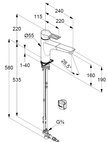
Dimensional drawing
