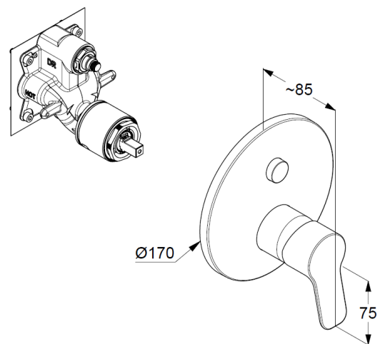
Dimensional drawing
