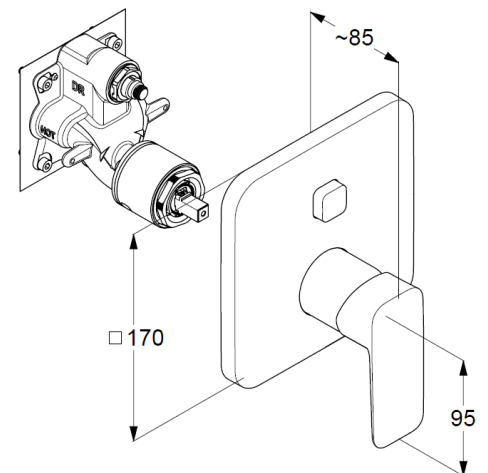
Dimensional drawing
