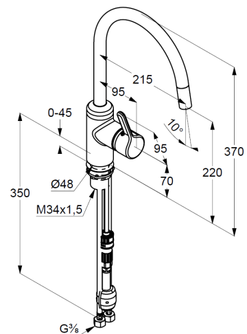
Dimensional drawing
