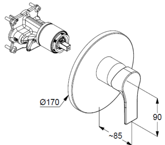
Dimensional drawing
